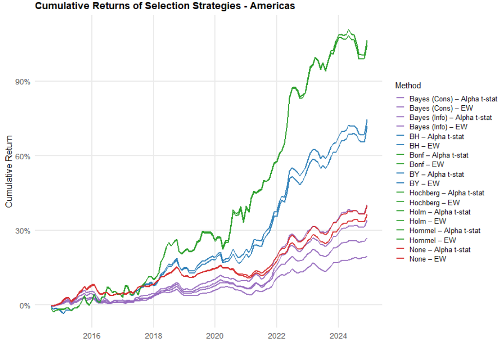
Figure 11: Cumulative returns of factor selection strategies in Americas. The figure reports the cumulative performance of portfolios constructed using different multiple-testing and Bayesian selection procedures, under equal-weight (EW) and alpha-weighted (t-statistic) schemes. Strategies are grouped by statistical approach: no adjustment (None), family-wise error rate control (FWER: Bonferroni, Holm, Hommel, Hochberg), false discovery rate control (FDR: Benjamini–Hochberg and Benjamini–Yekutieli), and Bayesian selection. Returns are compounded over time, allowing a direct comparison of long-run performance and the dynamic trade-offs between conservativeness and factor inclusion across methodologies.
