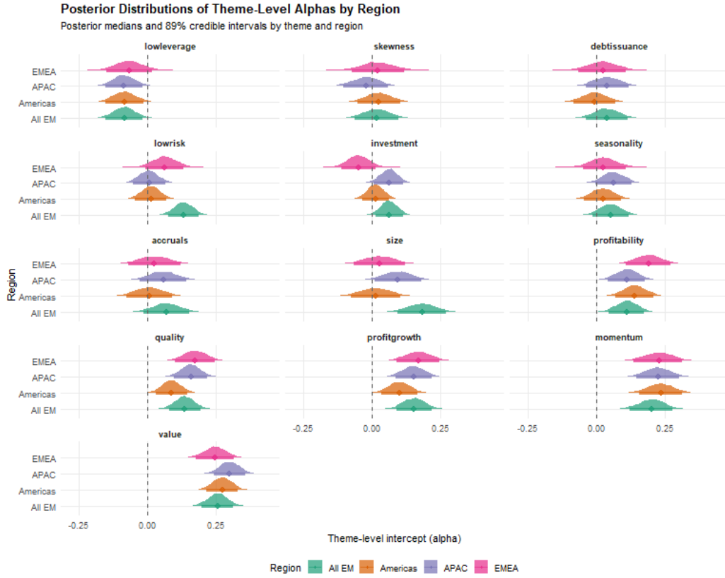
Figure 9: Posterior distribution for theme alphas across regions under conservative priors centered around 0 for \alpha_{c(i)} . All EM and specific regions distributions are represented each with a different color and 89% credible intervals are also displayed.
